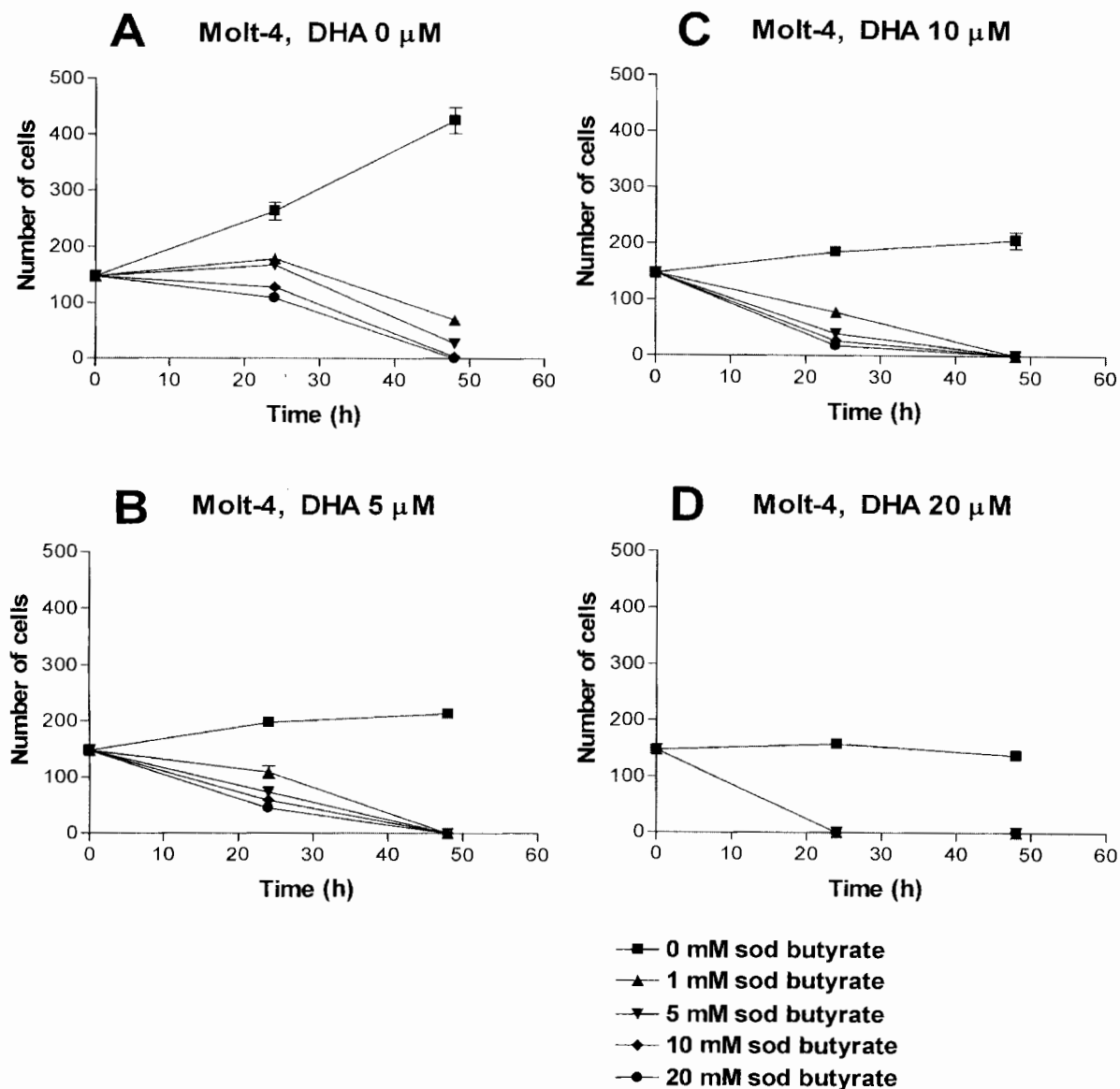
Figure 1. Graphs showing the number of Molt-4 cells (Mean \pm SD, N=3) at 0-, 24- and 48-hour time-points with different treatment combinations of DHA and sodium butyrate. Graphs show the effects of 0, 1, 5, 10 and 20 mM sodium butyrate added to cultures containing 0, 5, 10 and 20 \mu M DHA (Figures 1 A-D, respectively).
